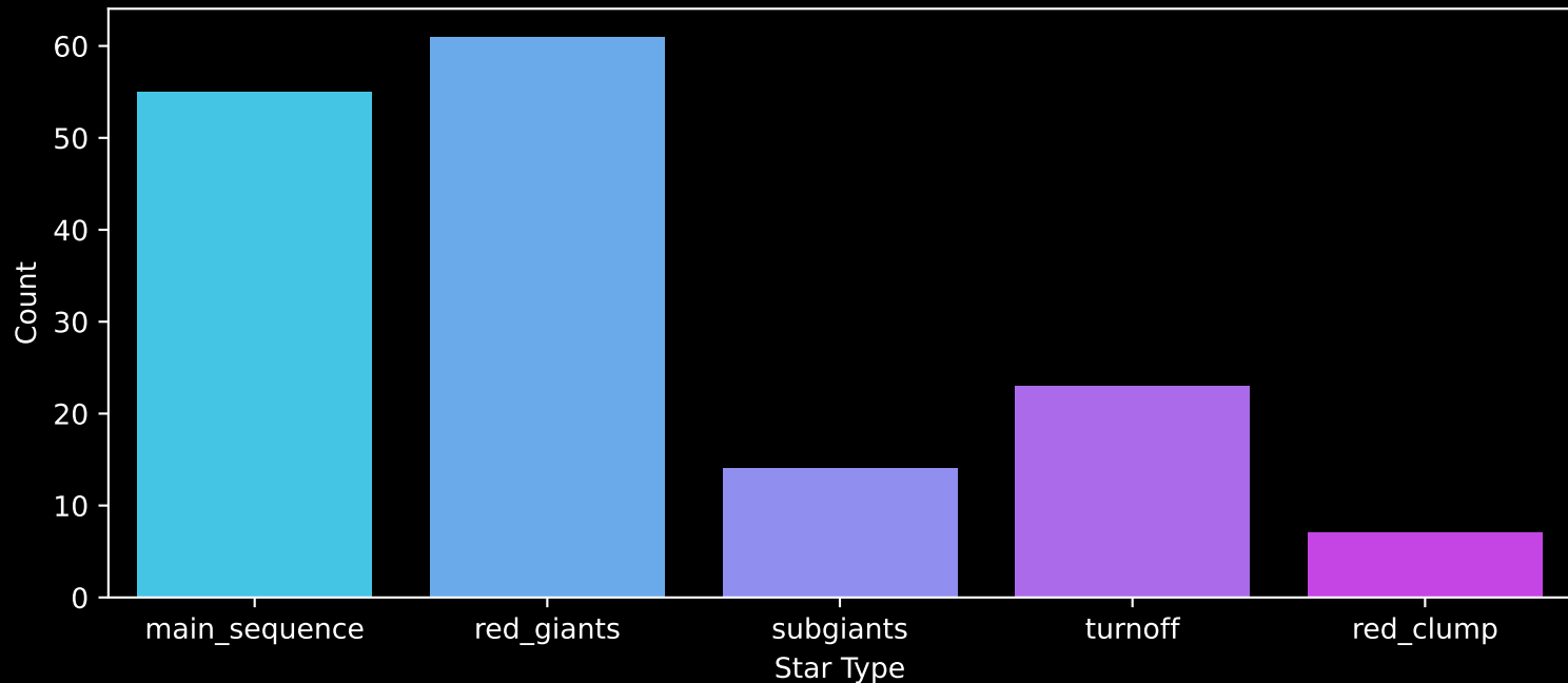
APOGEE DR17 Field: [041-28_MGA] Count plot of Star Type
