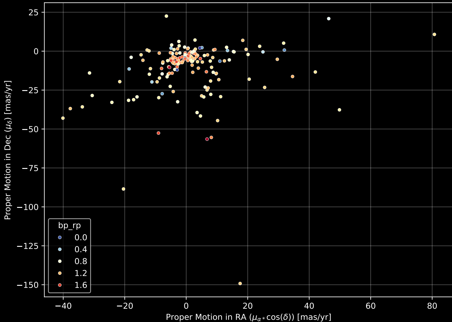
APOGEE DR17 Field: [041-28_MGA] Proper Motion Diagram (n= 160)
