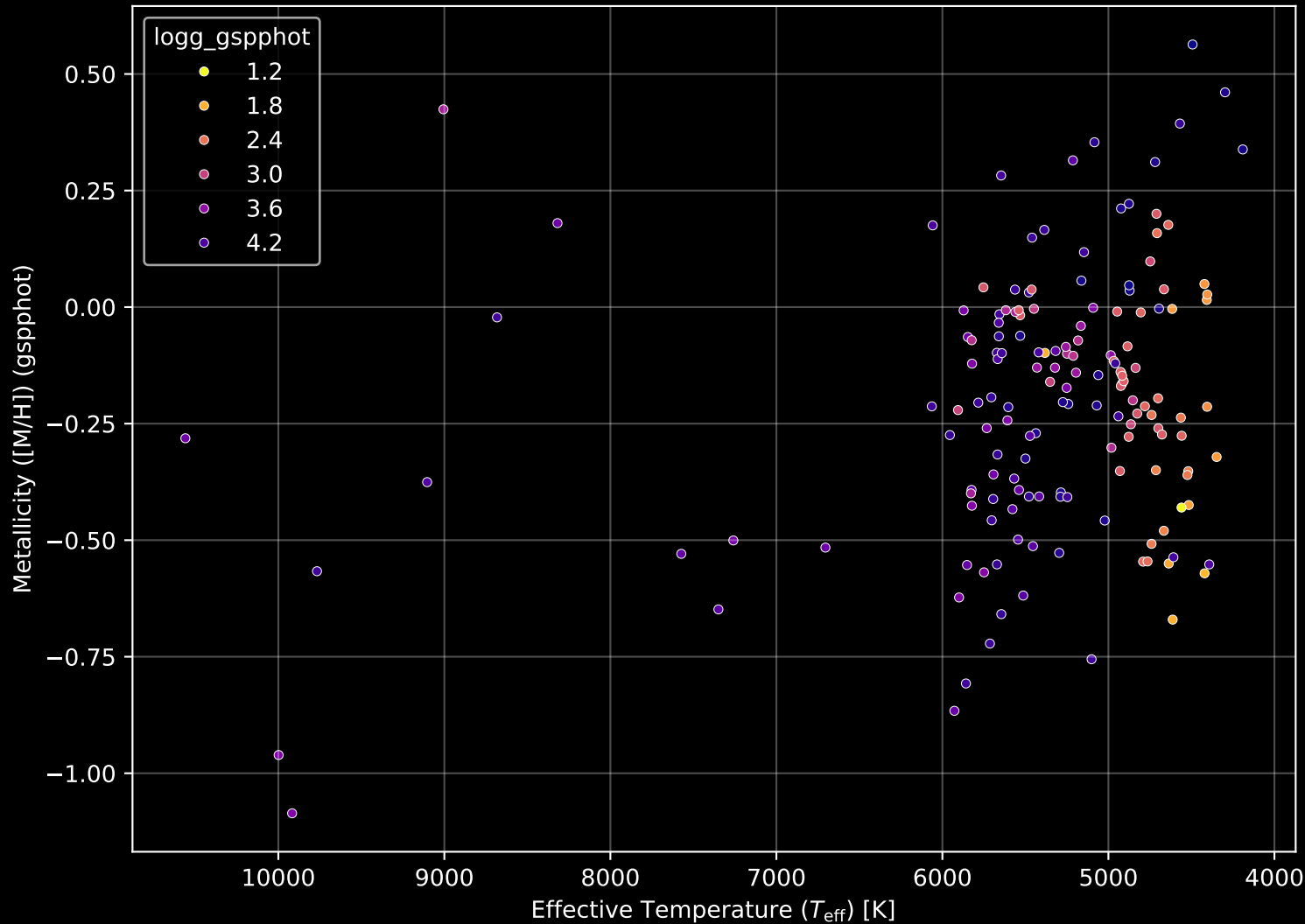
APOGEE DR17 Field: [041-28_MGA] Stellar Population Parameters (n= 160)
