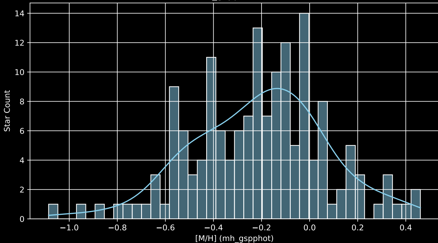
APOGEE DR17 Field: [041-28_MGA [M/H] (mh_gspphot) (n= 159)
