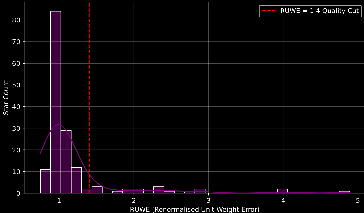
GAPOGEE DR17 Field [041-28_MGA] RUWE Distribution (n= 156)
