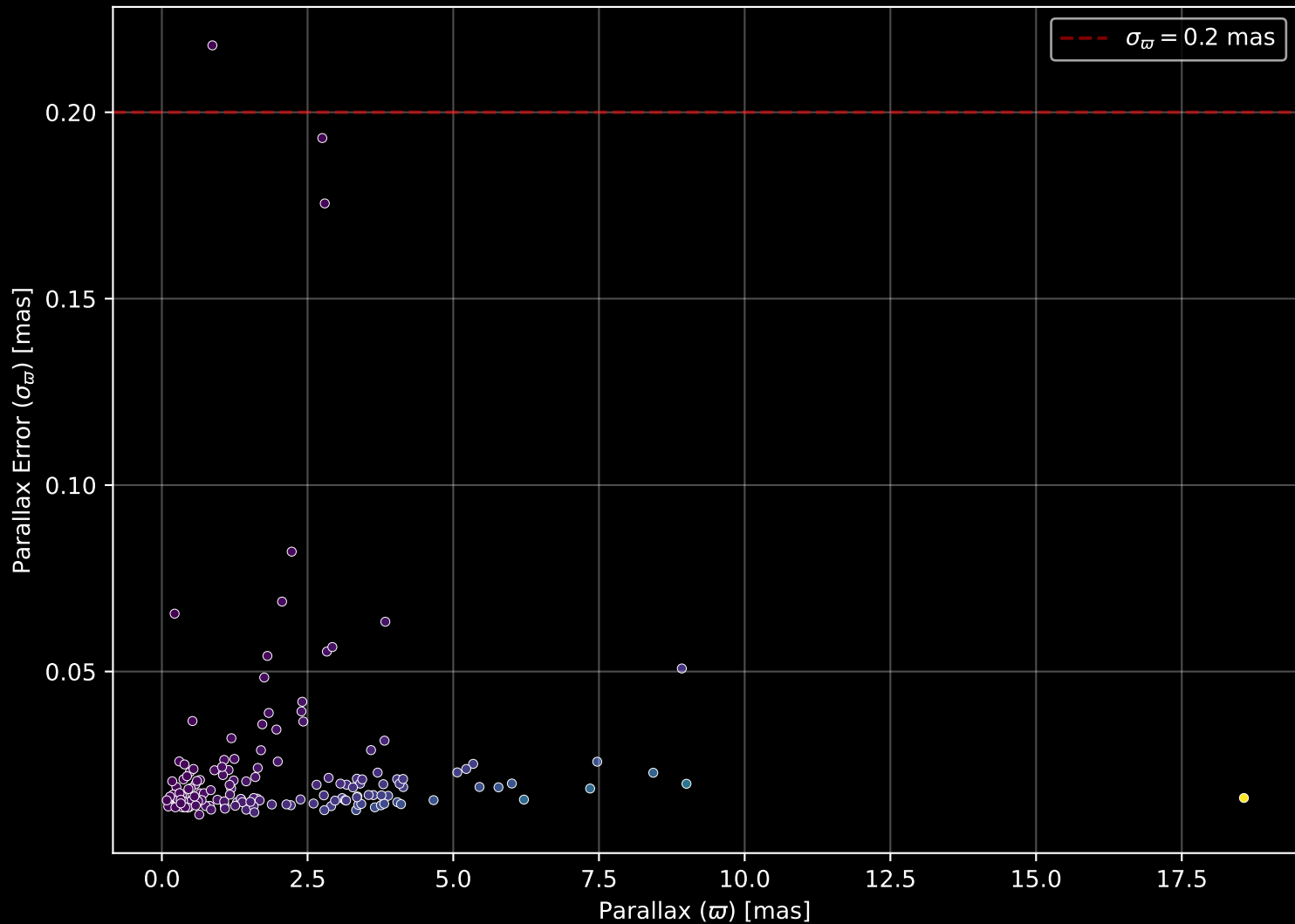
APOGEE DR17 Field: [041-28_MGA] Parallax Quality (n= 160)
