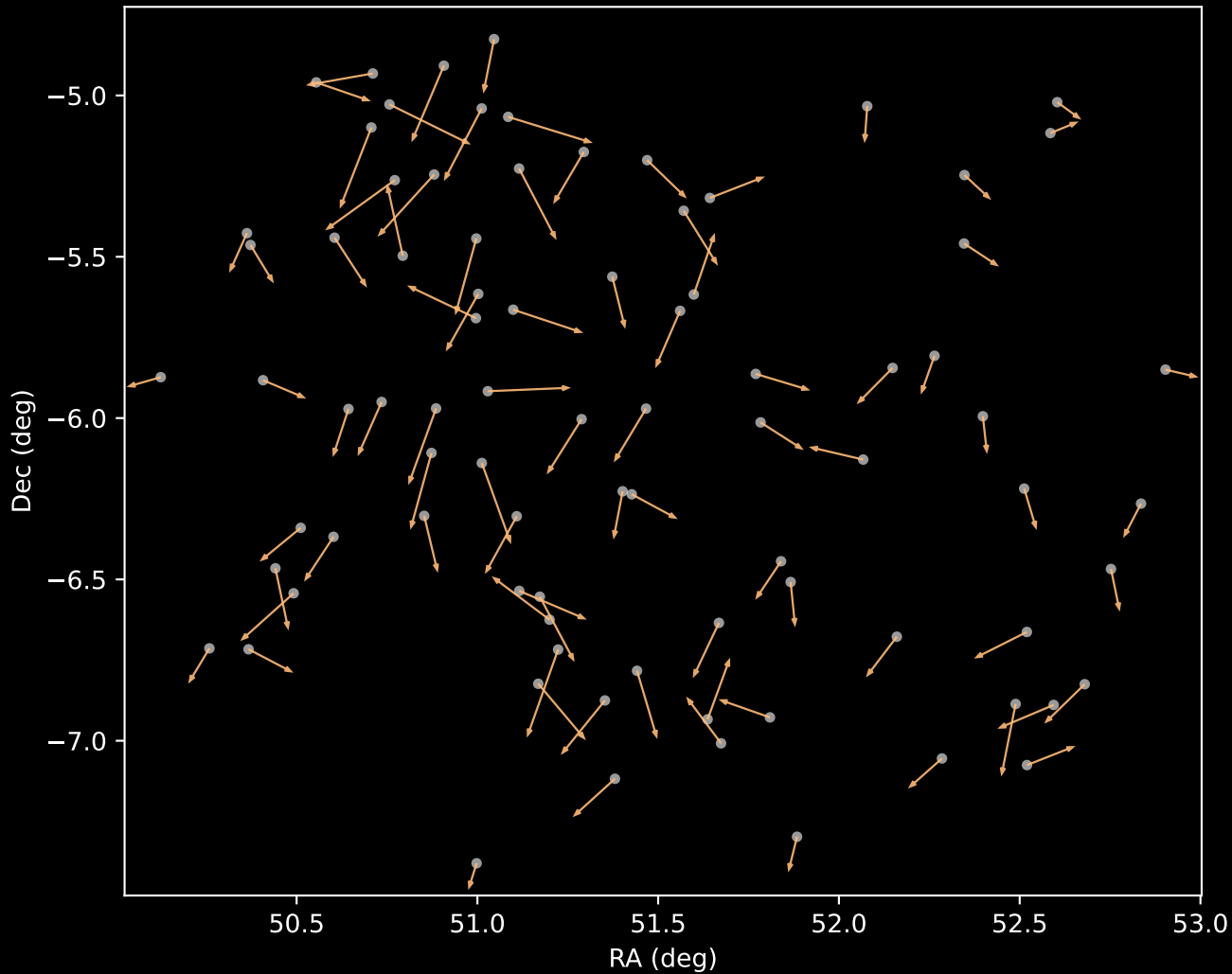
APOGEE DR17 Cluster 3 Proper Motion Vectors (n=84)
