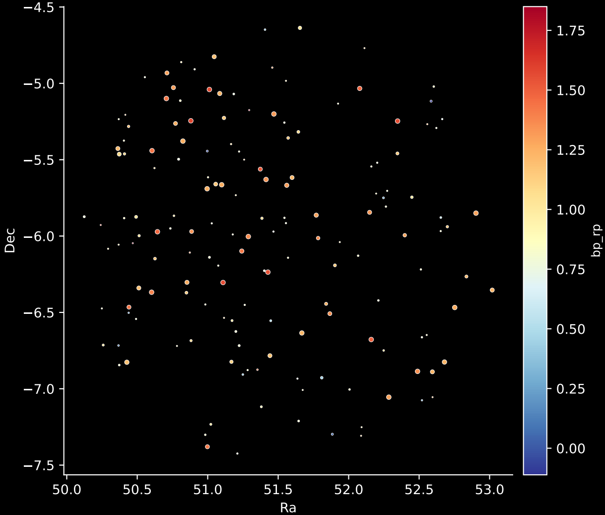
APOGEE DR17 Field: [041-28_MGA] Stars: 160
